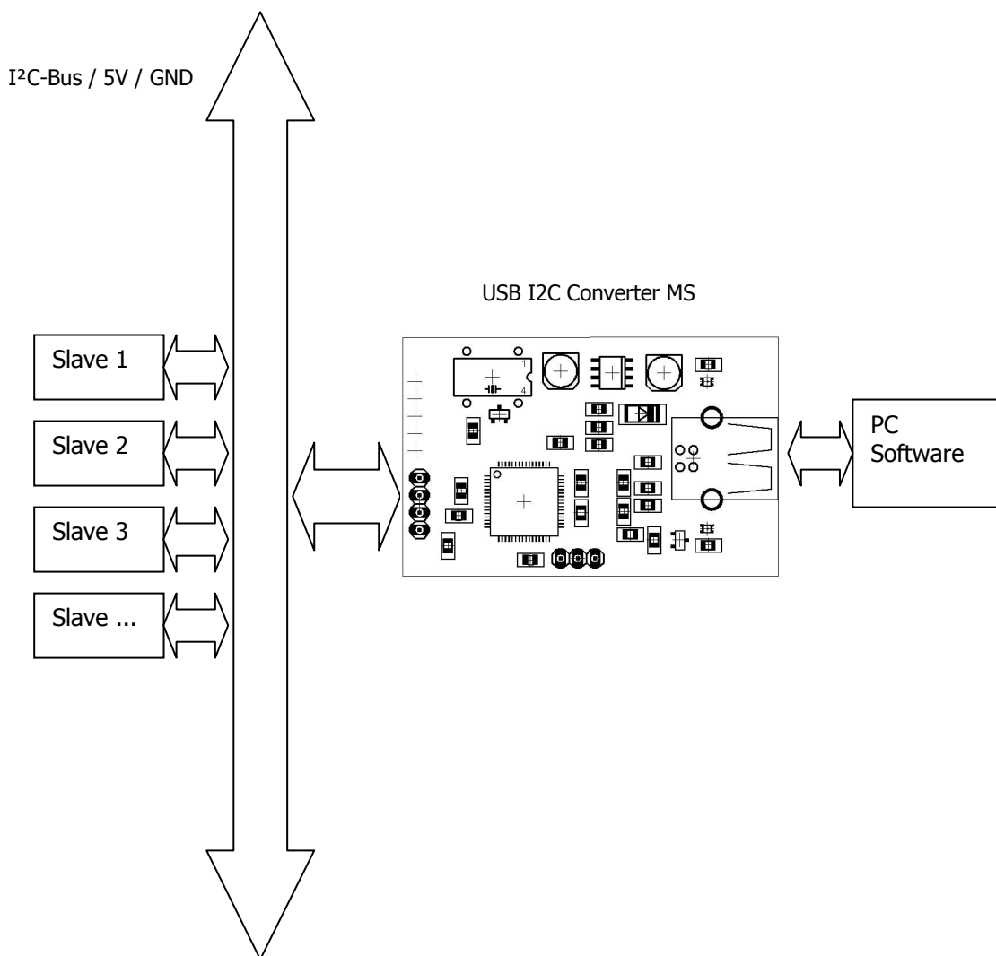
USB I2C Converter MS as Master
