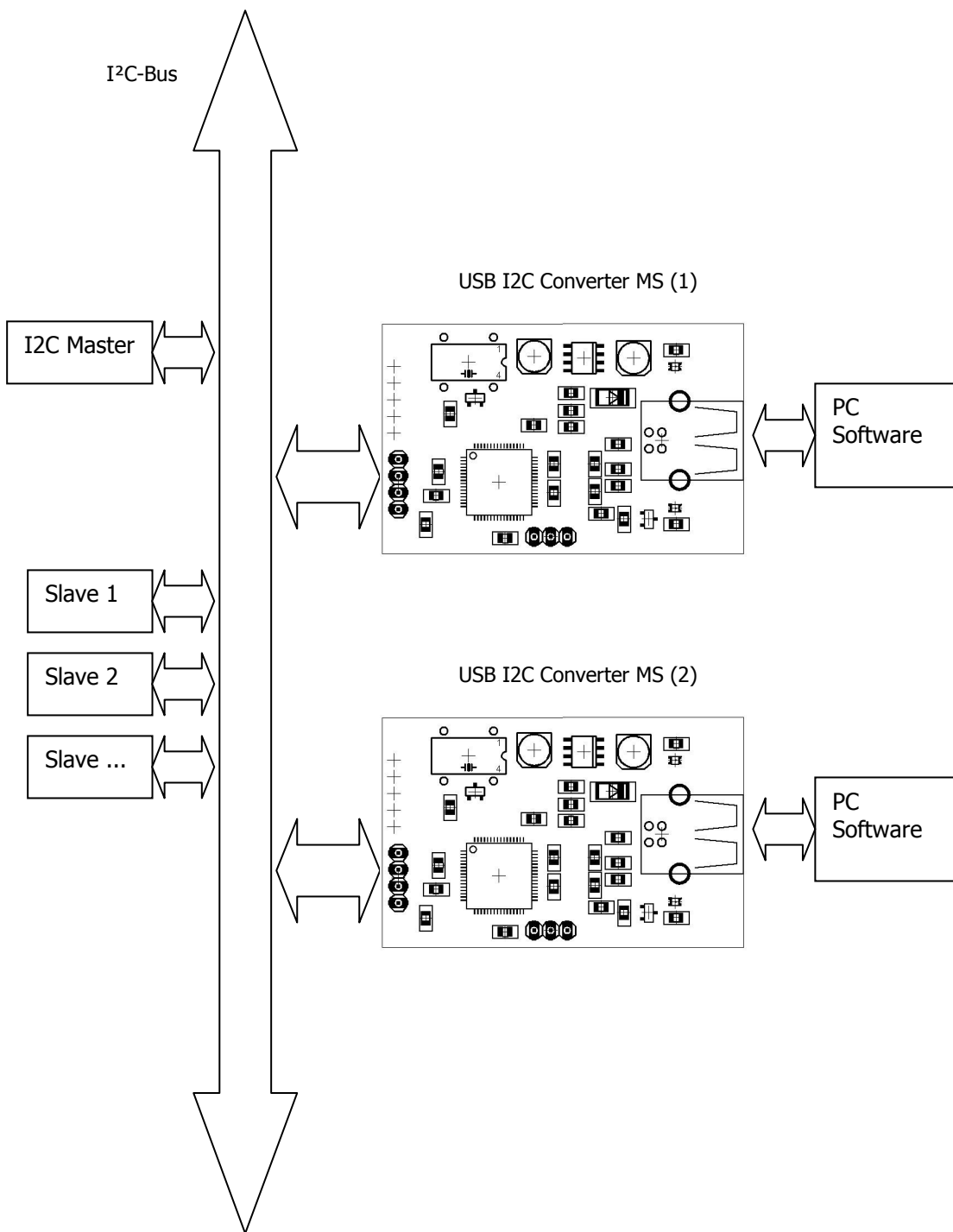
USB I2C Converter MS as Slave
